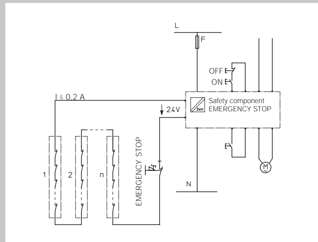
Signal transmitter with safety component and EMERGENCY STOP switch device.
