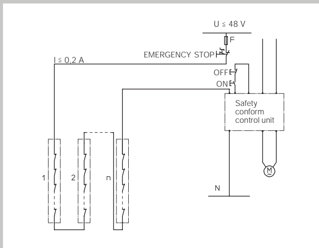
Signal transmitter included in the existing control.
