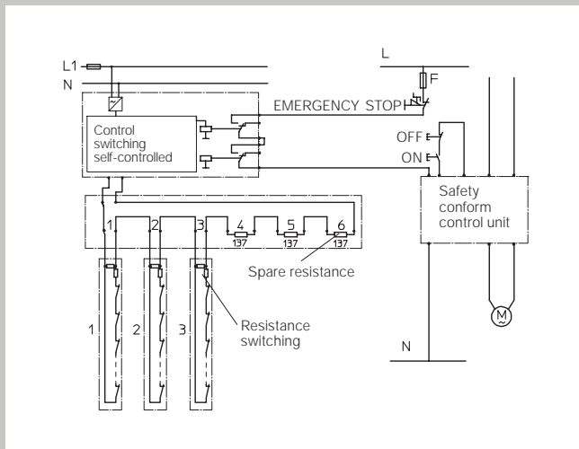
Signal transmitter with self-controlling control unit.
