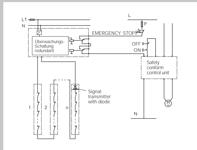
Signal transmitter with redundant control unit.
